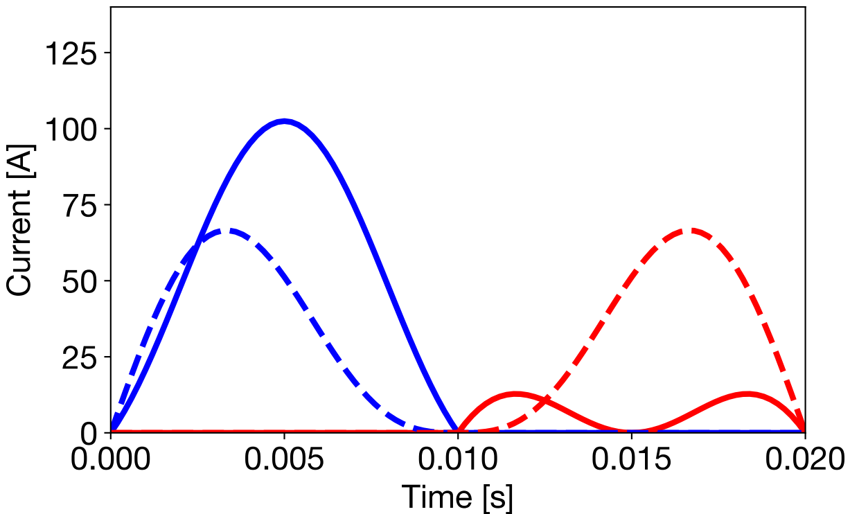
Instantaneous IGBT and diode currents
